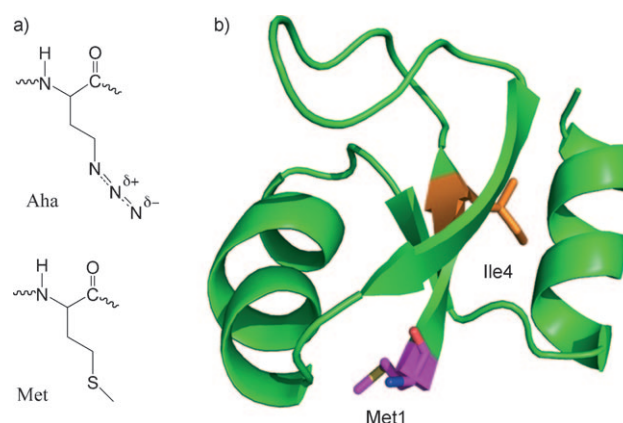
Figure 1. a) Structure of azidohomoalanine (Aha) and methionine (Met). b) A ribbon diagram of NTL9 showing the location of Met1 (pink) and Ile4 (orange). The diagram was generated using the pdb file 2HBA and the program Pymol.
